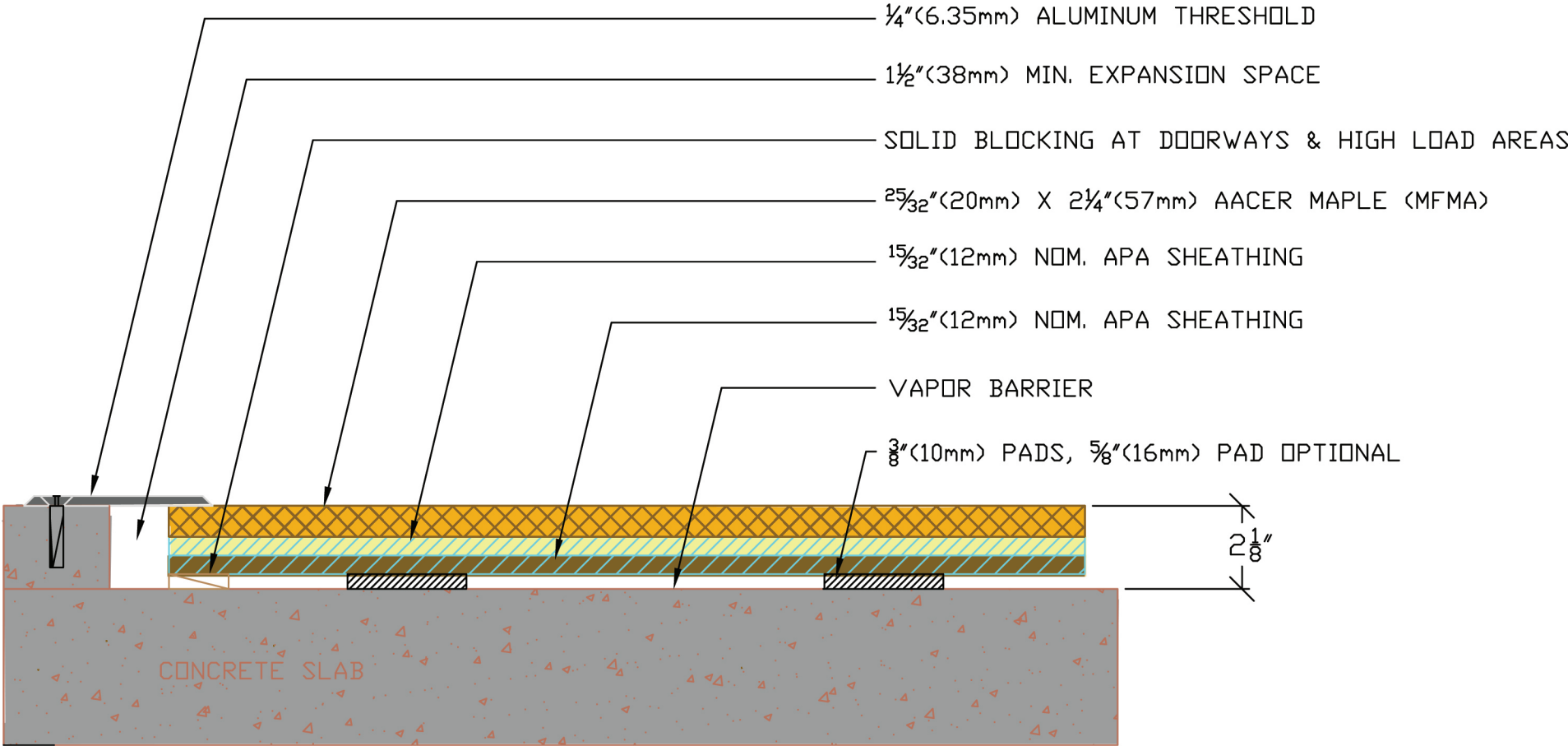
Threshold Detail
