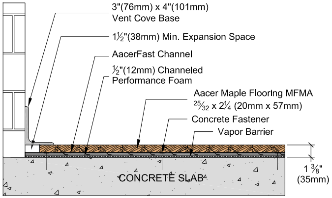
Wall Base
