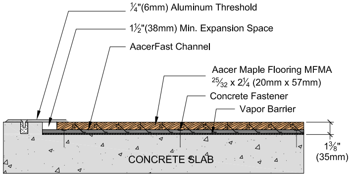
Threshold
