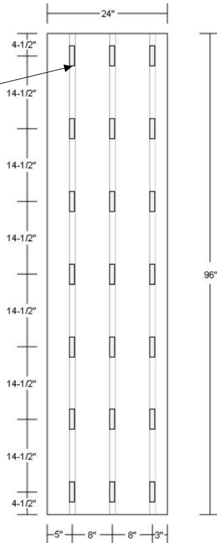
15/32" BOTTOM SECTION
