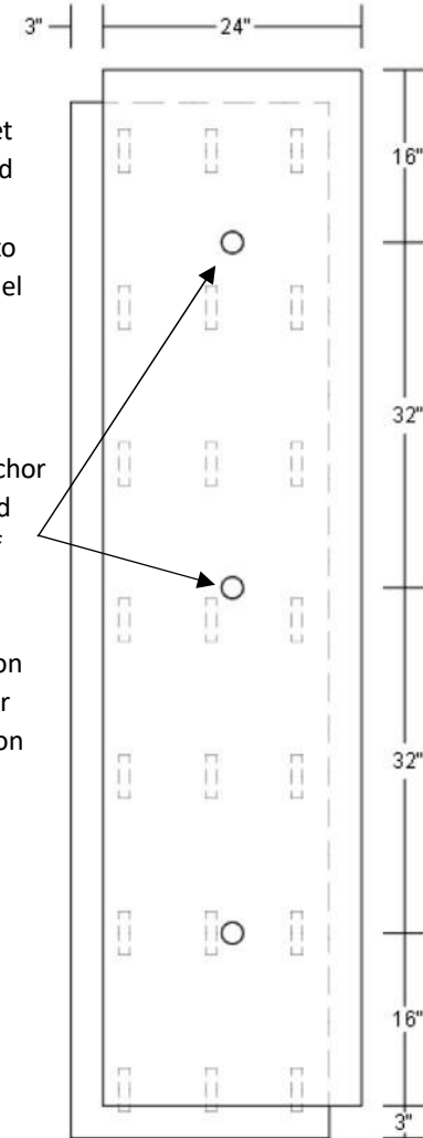
ASSEMBLED PANEL
