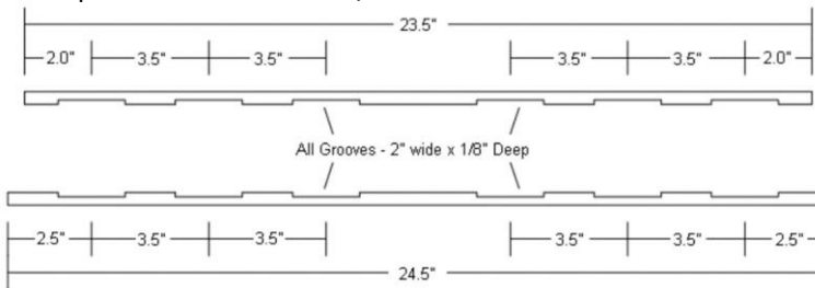
Bottom Subfloor Section 24-1/2" x 96"
