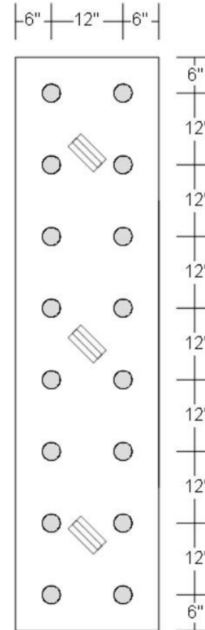
Top View - Resilient Pad Locations
