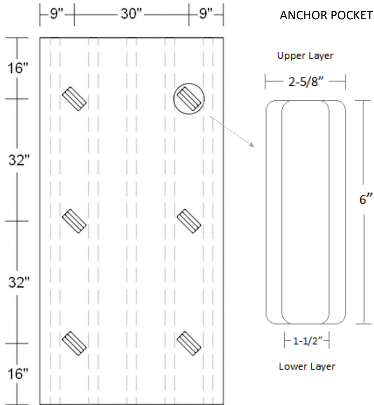
Top View - Anchor Pocket Locations
